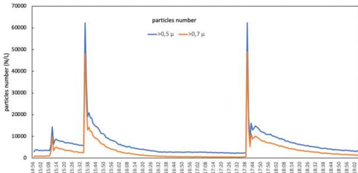
Fig. 4. Particles number concentration during the measuring period (N/L = number of particles per liter).
