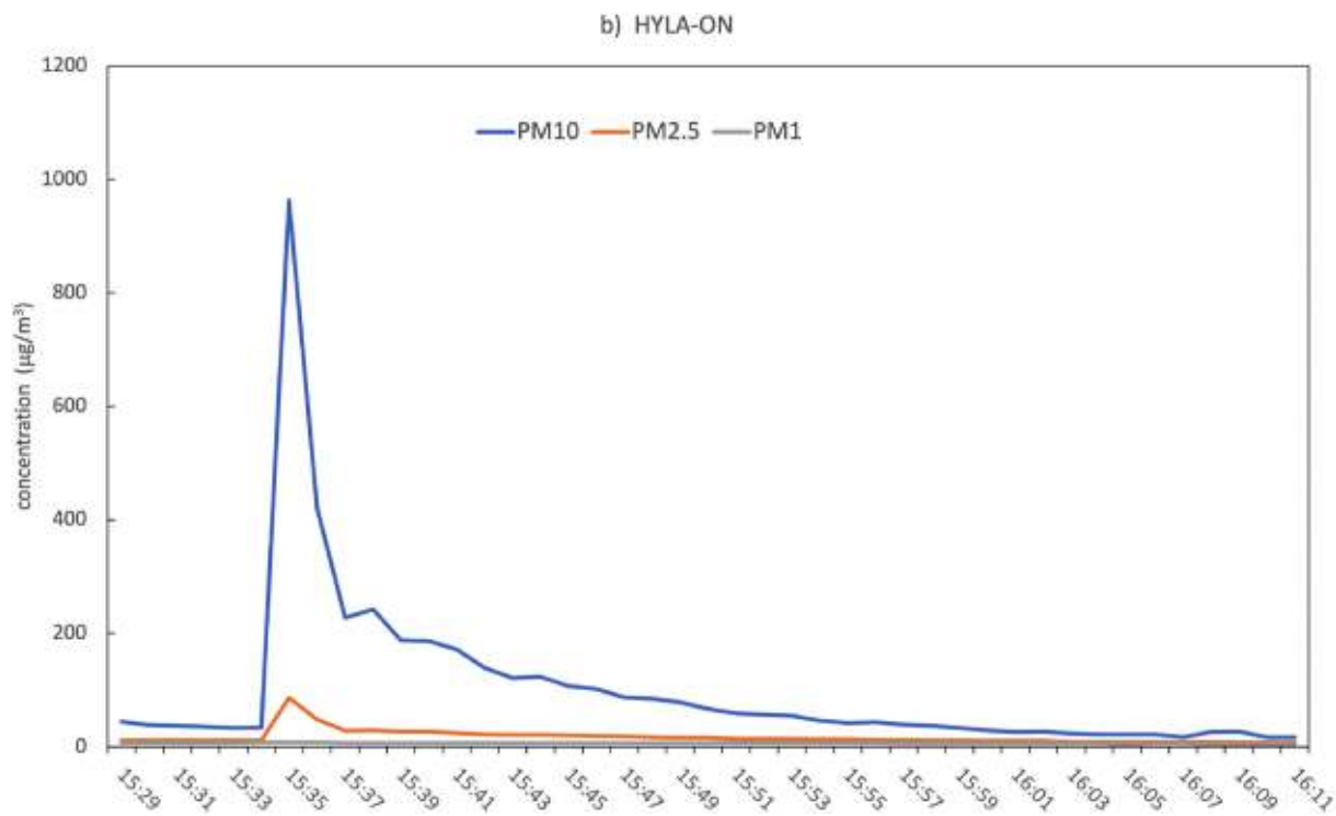
Fig. 2. PM concentration with the HYLÀ device switched off (2a) and on (2 b).
