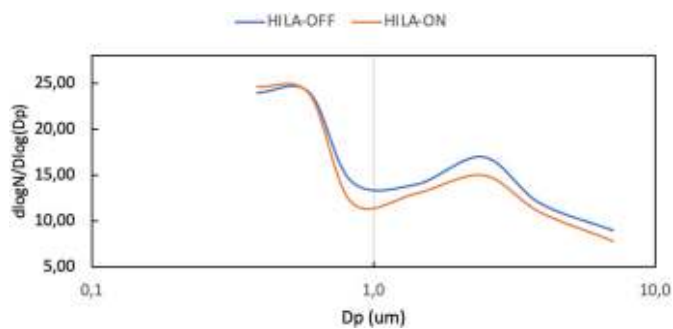
Fig. 5. Particle number distribution calculated as d\log N/d\log(Dp) .
