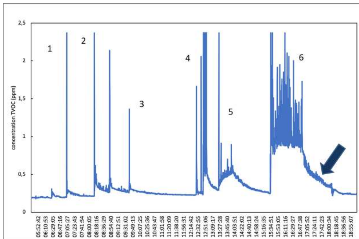
Fig. 6. TVOC concentration during the experiment (ppm).
