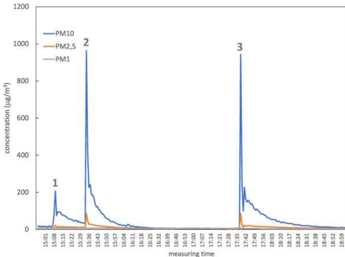
Fig. 1. PM10, PM2.5 and PM1 concentration trends during the measurement period.
