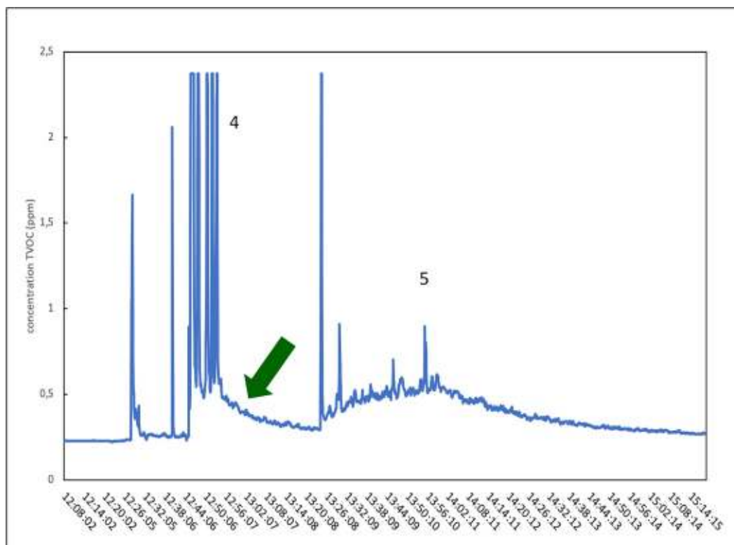
Fig. 7. TVOC concentrations during the experiment (ppm): detail of Fig. 6.
